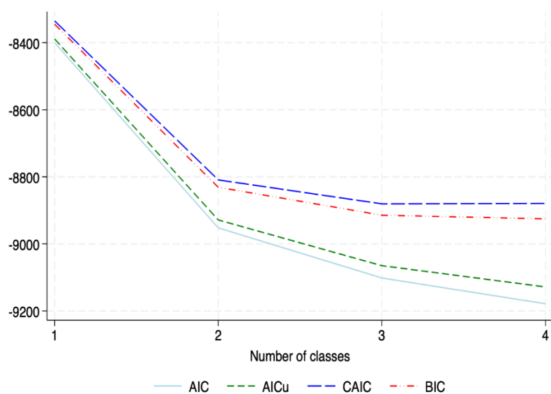
Figure 3: Specification tests for determining the number of regimes.
