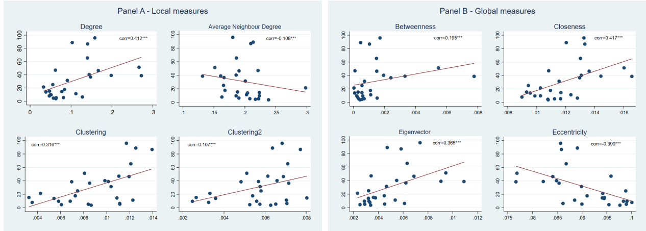
Figure 3: Scatter plot for INF/POP and local versus global centrality measures
