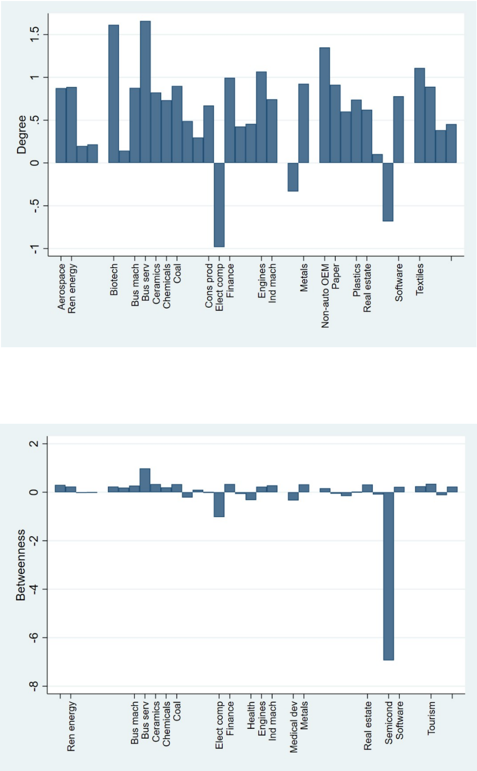
Figure A2 - Estimated coefficients of other NC measures for different sectors, DEATH/POP
