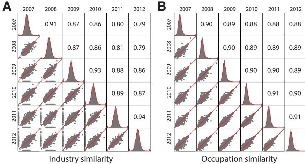
Figure 5: Pearson correlation of the relatedness coefficient across different years.
